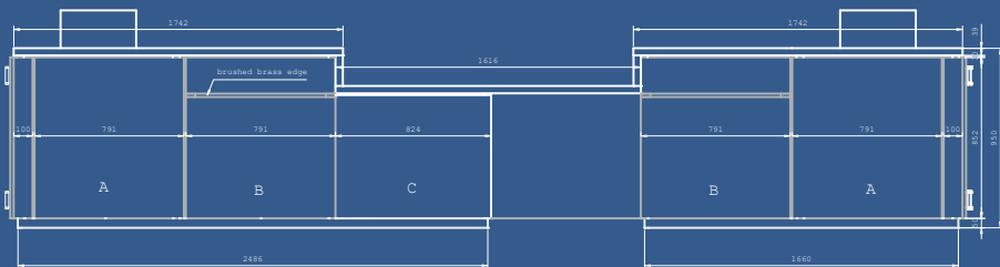
Front view M(1:10)
