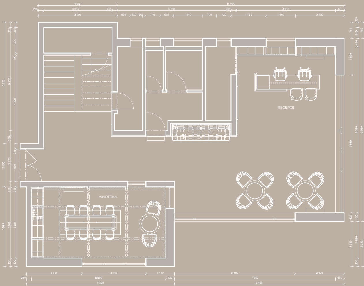
Floor plan
